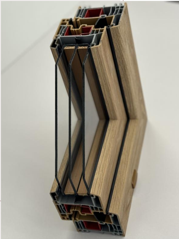
Triple glazing
